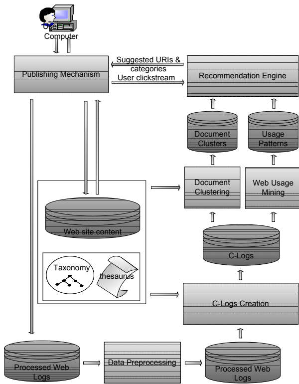
Figure 1: System architecture
