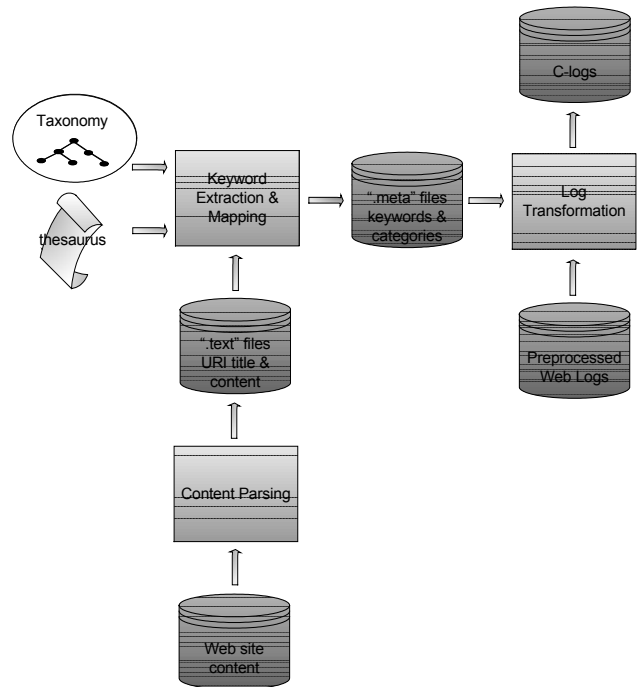
Figure 2: C-logs creation
